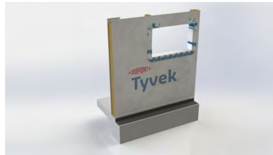
4. Completed flashing
