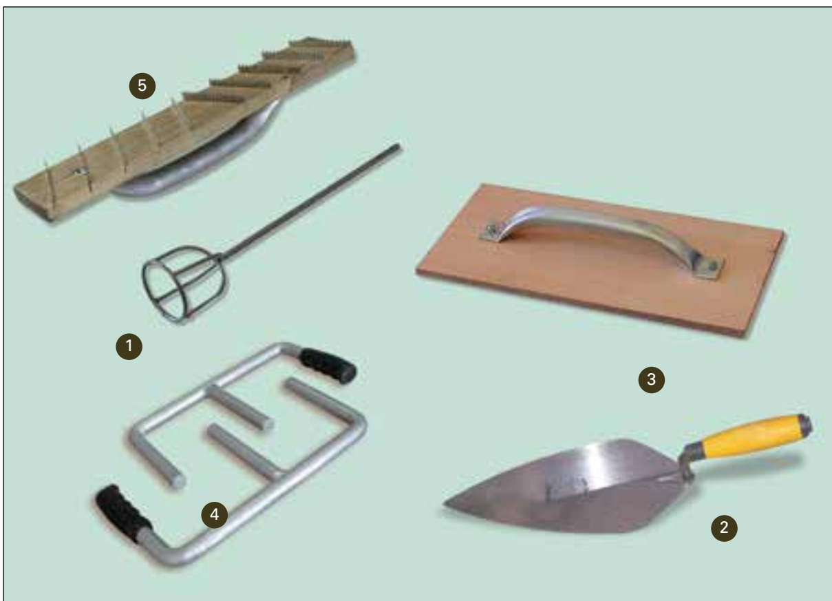
Figure 4.2.1 The Basic Tools and Equipment Requirements
