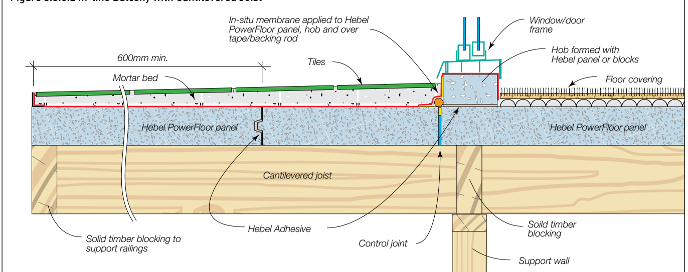
Figure 3.3.8.2 In-line Balcony with Cantilevered Joist
