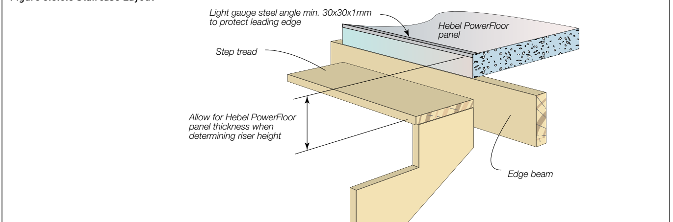
Figure 3.3.8.3 Staircase Layout
