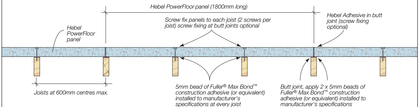
Figure 3.3.1.2 Fixing Layout
