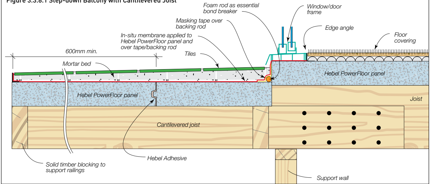
Figure 3.3.8.1 Step-down Balcony with Cantilevered Joist
