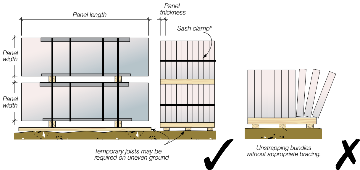
Figure. 4.1.1 Stacking Packs of Hebel PowerFloor
