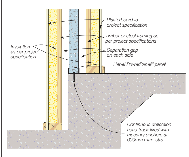
Figure 1.10.2.5 Base detail at stepped slab - Option 2
