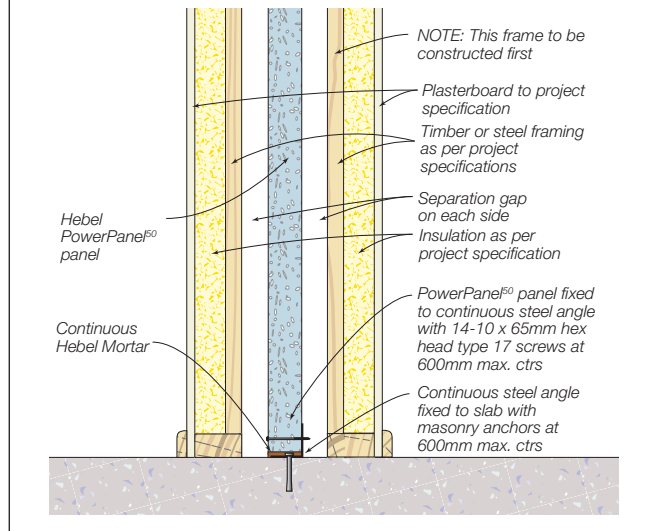
Figure 1.10.2.2 Base connection - Continuous steel angle
