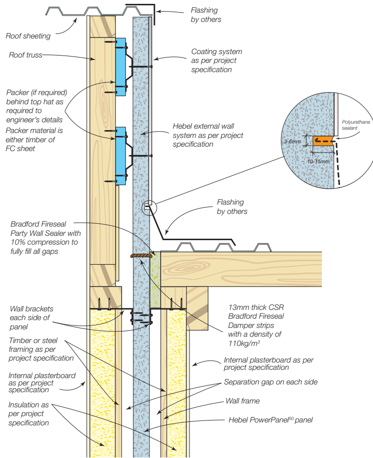
Figure 1.10.4.11 Intertency wall to Hebel external walls
