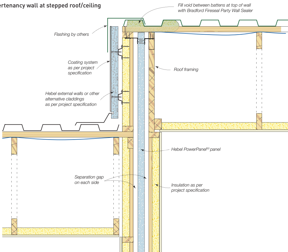
Figure 1.10.4.13 Hebel Intertency wall at stepped roof/ceiling
