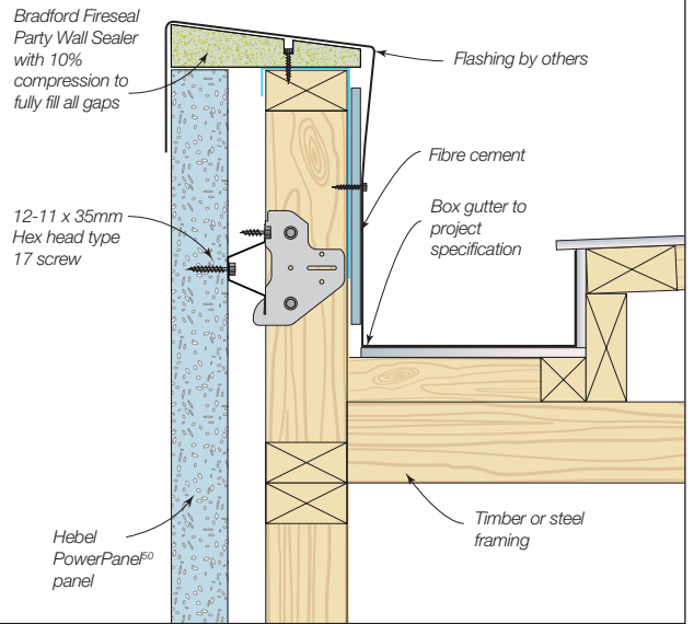
Figure 2.10.3.2 Typical Dual Zero Boundary roof eave detail
