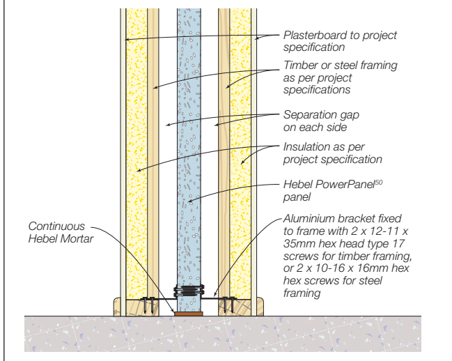
Figure 1.10.2.3 Base connection - Wall bracket
