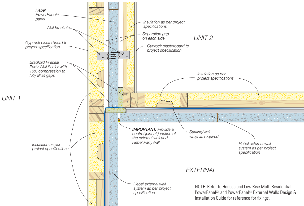
Figure 1.10.4.5 External wall corner junction for PowerPanel 50 Intertency Walls - Option 1
