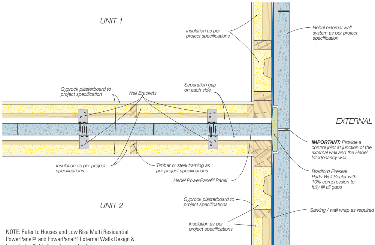
Figure 1.10.4.1 External wall junction for PowerPanel 50 Intertency Walls
