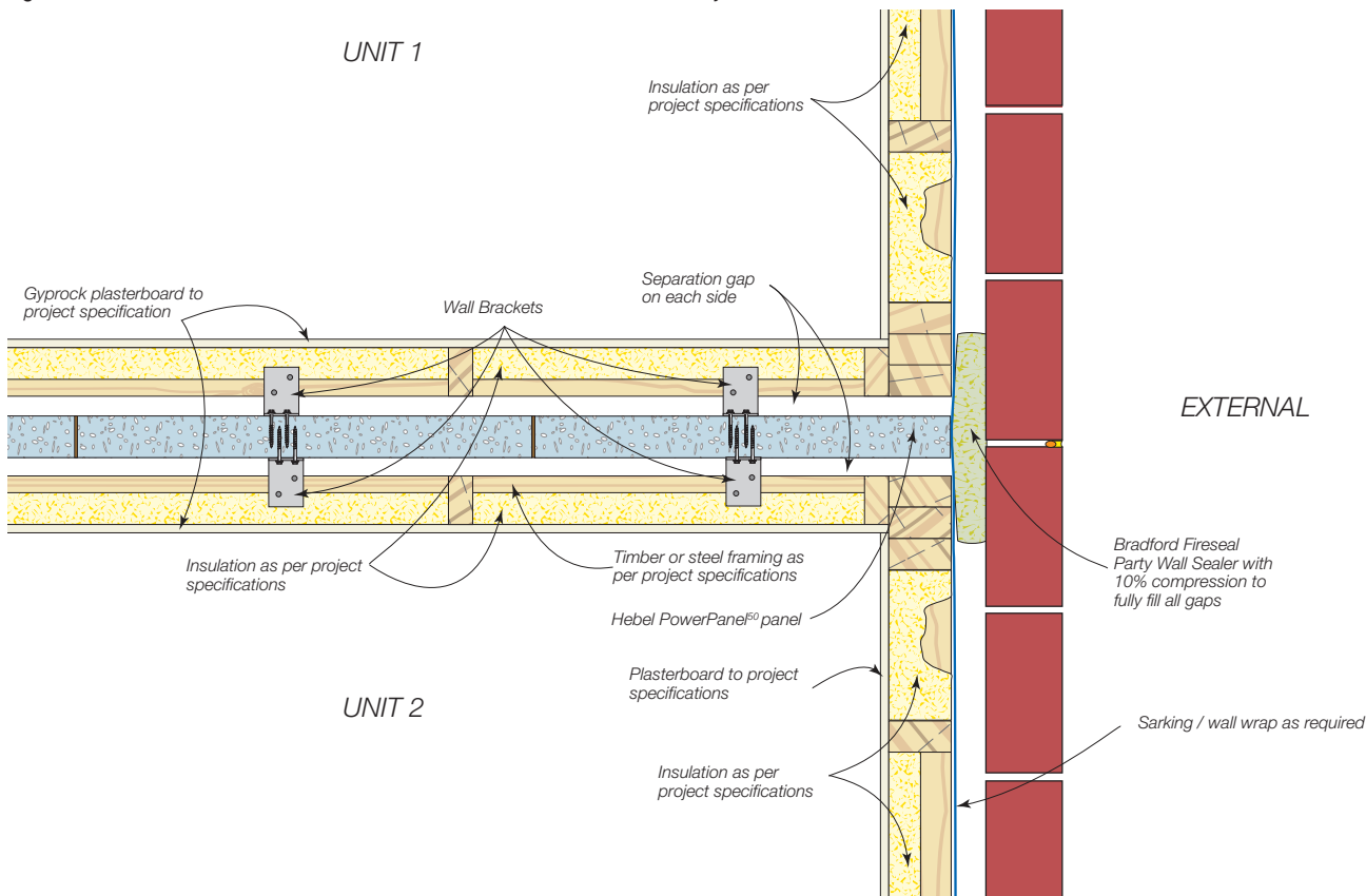
Figure 1.10.4.2 Junction of Brick veneer and PowerPanel 50 Intertency walls
