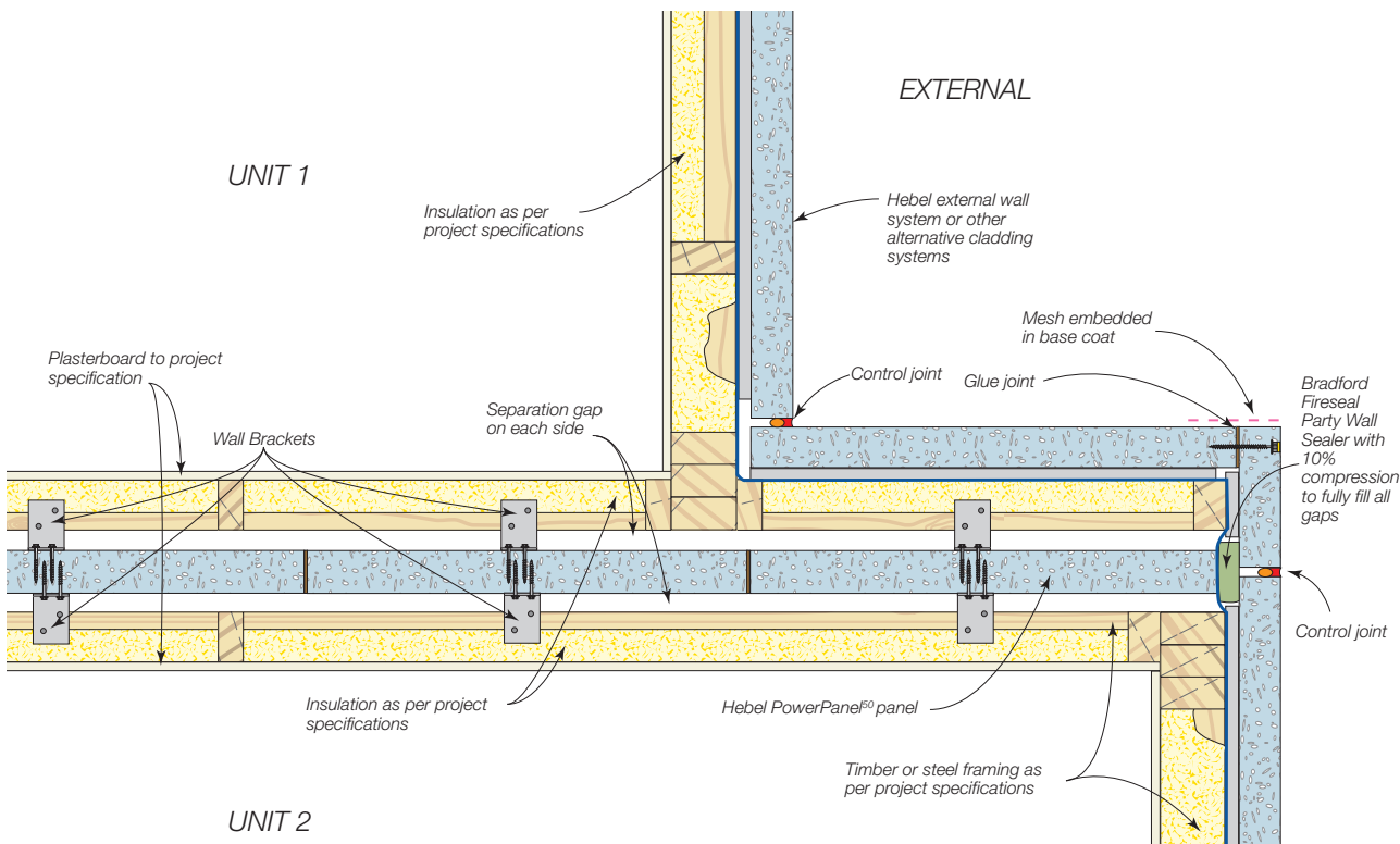
Figure 1.10.4.6 External wall corner junction for PowerPanel 50 Intertency Walls - Option 2
