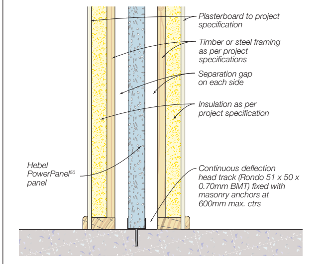
Figure 1.10.2.1 Base connection - Continuous deflection head track
