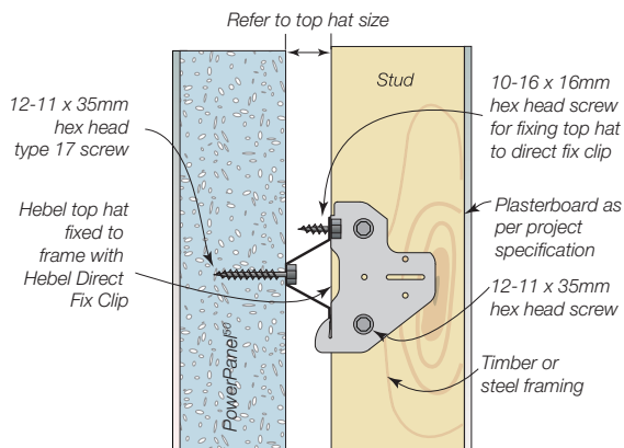
Figure 2.10.2.2 Hebel PowerPanel 50 Dual Zero Boundary Walls fixing detail – Hebel panel internally fixed
