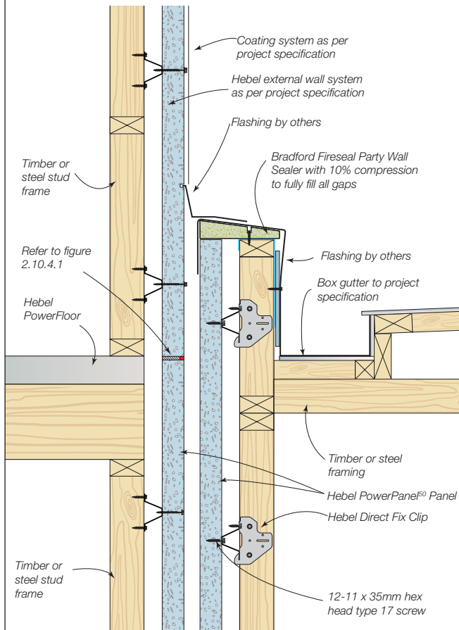
Figure 2.10.3.3 Dual Zero Boundary Wall detail to Hebel External Walls
