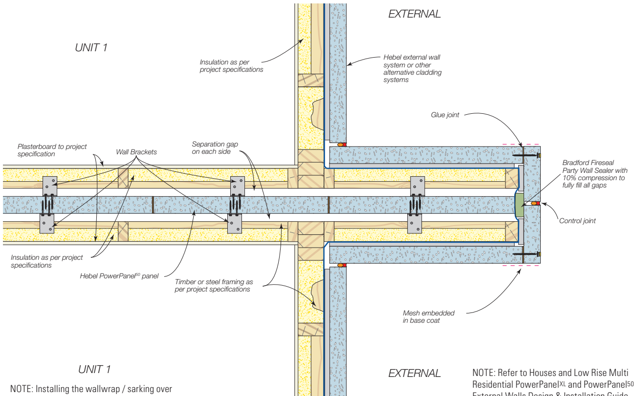
Figure 1.10.4.8 Nib junction detail of PowerPanel 50 Intertency wall and external wall system
