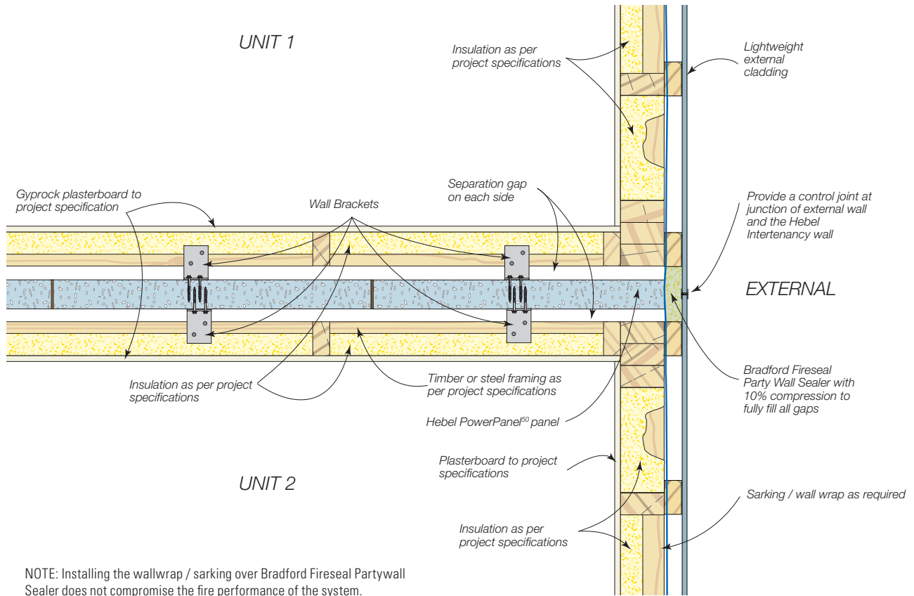
Figure 1.10.4.3 Junction of lightweight external cladding and PowerPanel 50 Intertency walls
