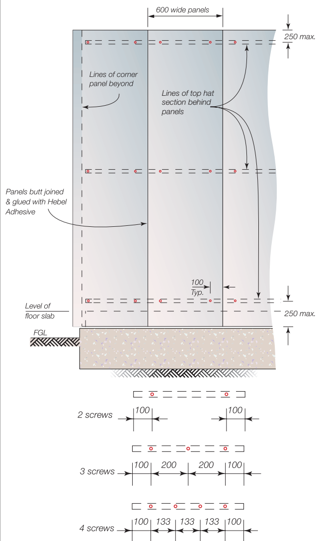
Figure 2.10.2.3 Screw layout drawing
