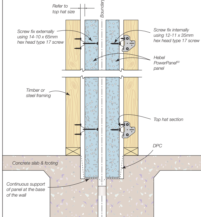
Figure 2.10.2.4 Typical Dual Zero Boundary Wall section detail
