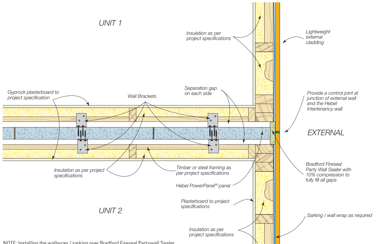
Figure 1.10.4.4 Junction of lightweight external cladding (direct fixed to studs) and PowerPanel 50 Intertency walls
