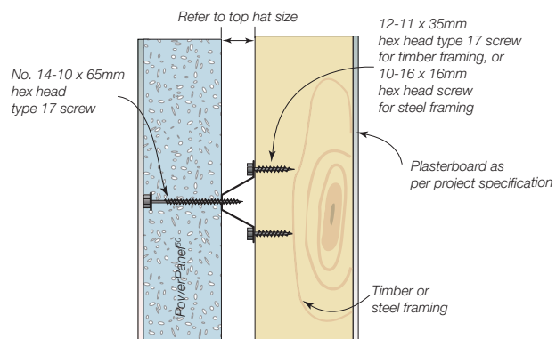
Figure 2.10.2.1 Hebel PowerPanel 50 Dual Zero Boundary Walls fixing detail – Hebel panel externally fixed
