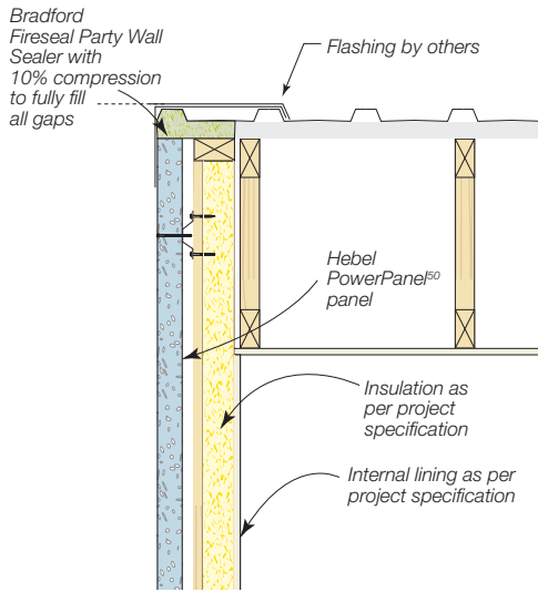
Figure 2.10.3.1 Typical Dual Zero Boundary Wall to roof detail
