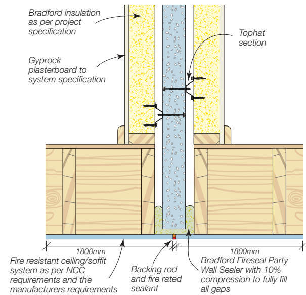
Figure 1.10.9.2 Cantilevered Soffit
