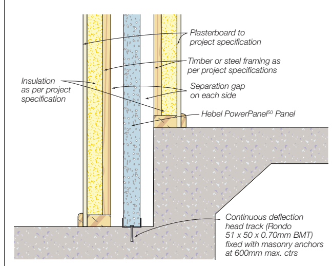
Figure 1.10.2.4 Base detail at stepped slab - Option 1
