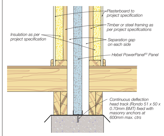
Figure 1.10.2.6 Base detail at subfloor
