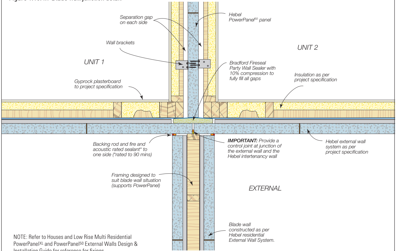
Figure 1.10.4.7 Blade wall junction detail
