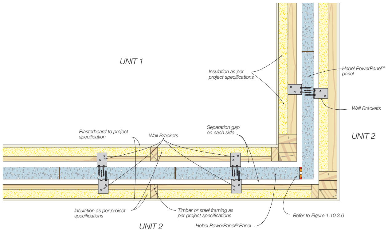
Figure 1.10.4.9 Corner junction detail for PowerPanel 50 Intertency walls
